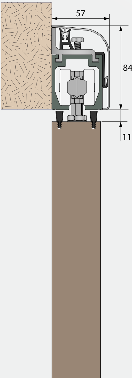
CROSS SECTION OF TOP PART
