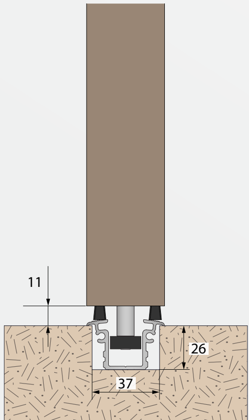
CROSS SECTION OF BOTTOM PART
